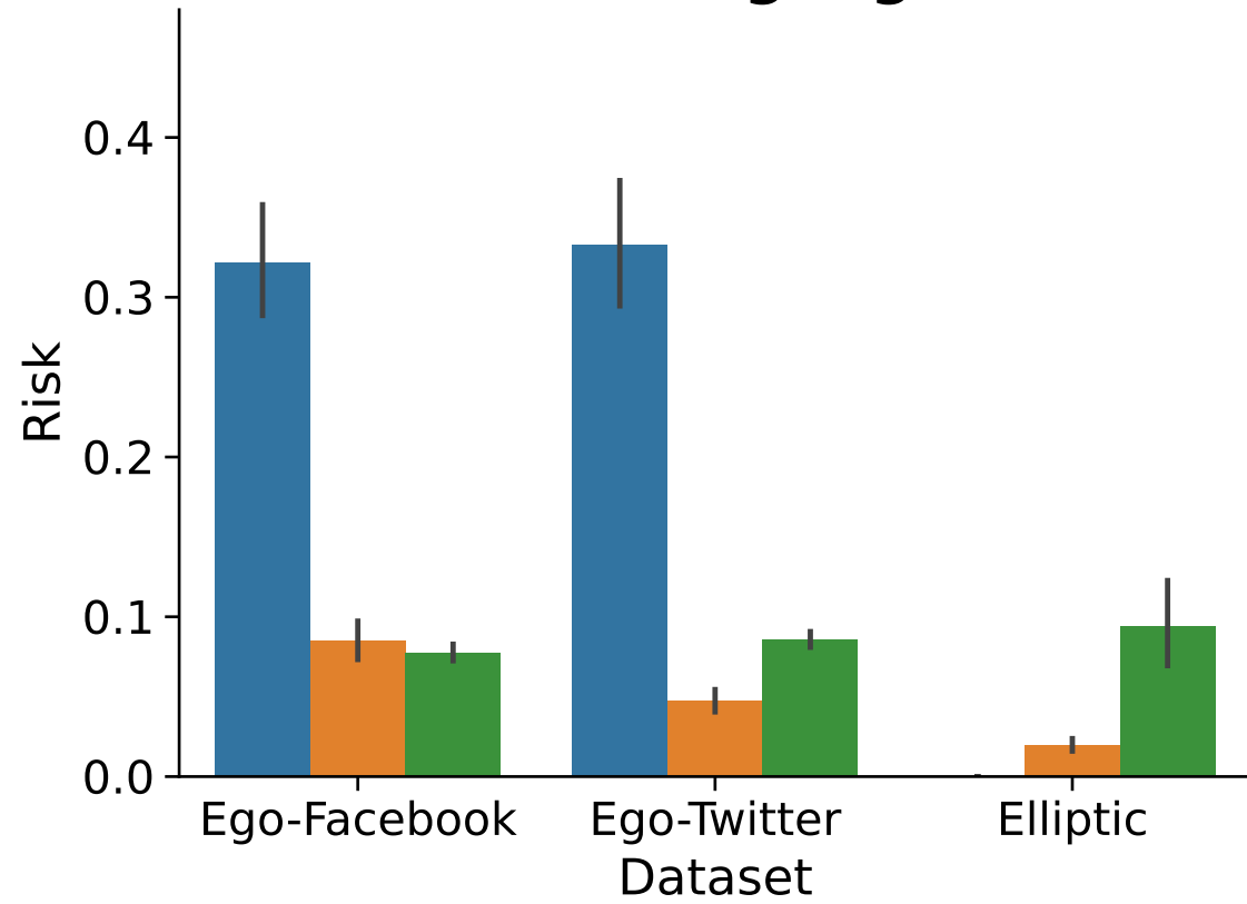
Attack: singling-out
