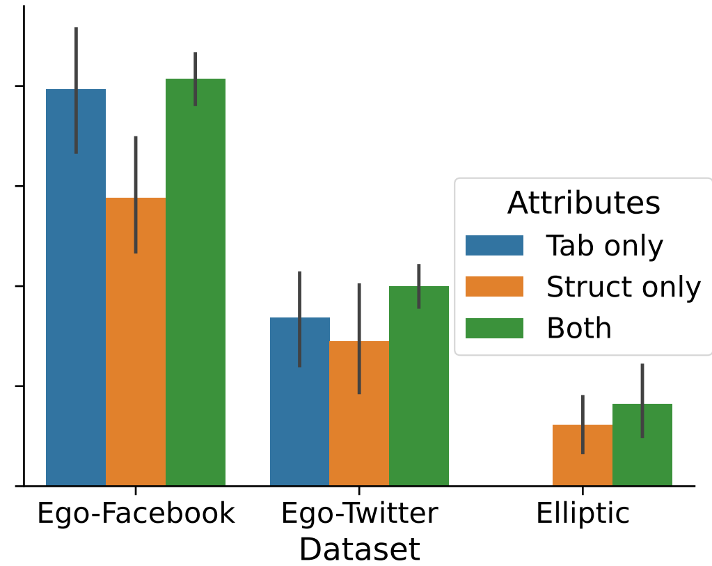
Attack: inference
