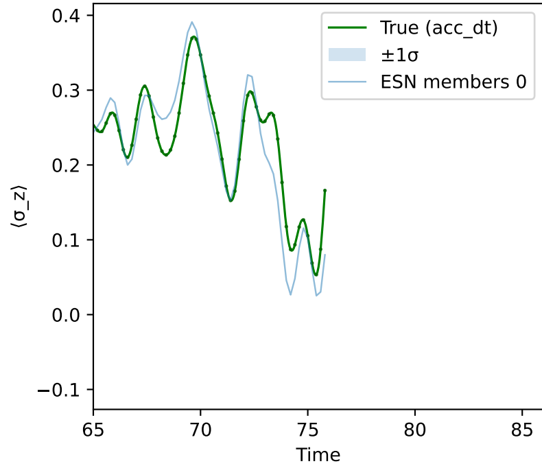
N=5, Qubit=0
