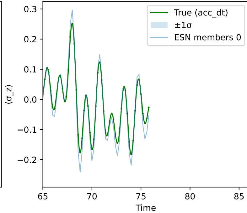
N=5, Qubit=2
