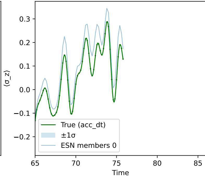
N=5, Qubit=1
