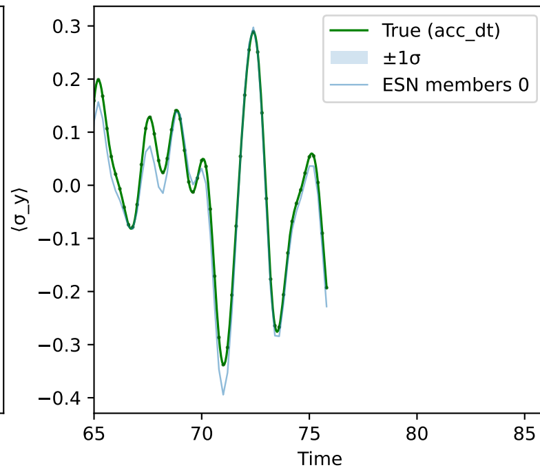
N=5, Qubit=2
