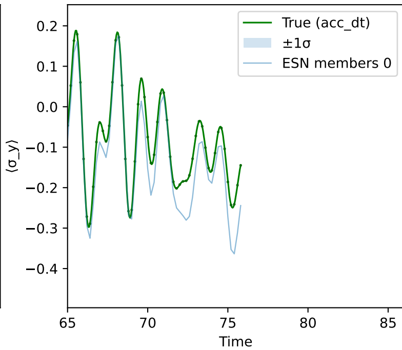
N=5, Qubit=1
