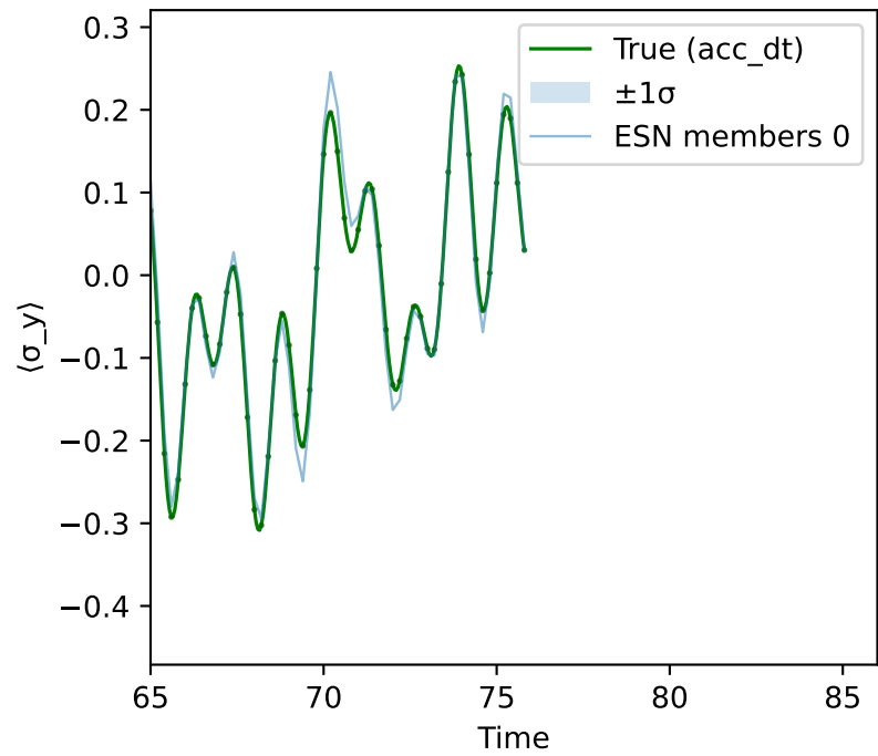
N=5, Qubit=0
