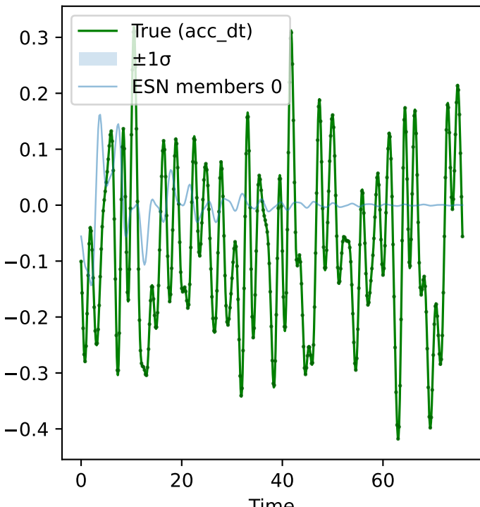
N=5, Qubit=1
