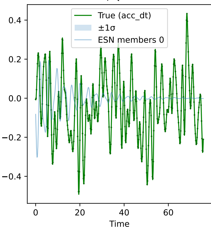
N=5, Qubit=3
