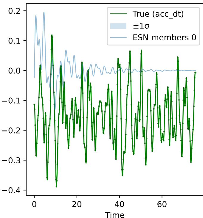
N=5, Qubit=3
