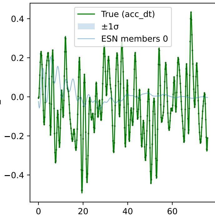
N=5, Qubit=4
