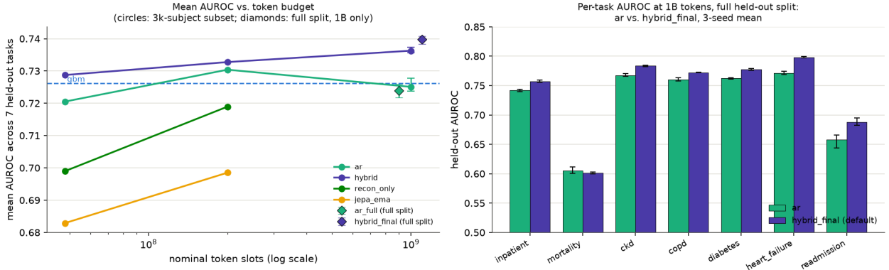
Figure 7: Left: mean AUROC against token budget ( \log x ) for ar , the hybrid, recon_only and jepa_ema on the 3,000-subject held-out subset (circles), with gbm as a horizontal reference; the subset 1B ar /hybrid points are 3-seed means with a min-max error bar. The diamonds at 1B are the full-held-out-split (Section 6.10) 3-seed means for ar and hybrid_final , offset in x so they do not overlap the subset circles. Right: per-task AUROC at 1B tokens on the full held-out split, ar against hybrid_final , paired bars, each a 3-seed mean with a min-max whisker.
