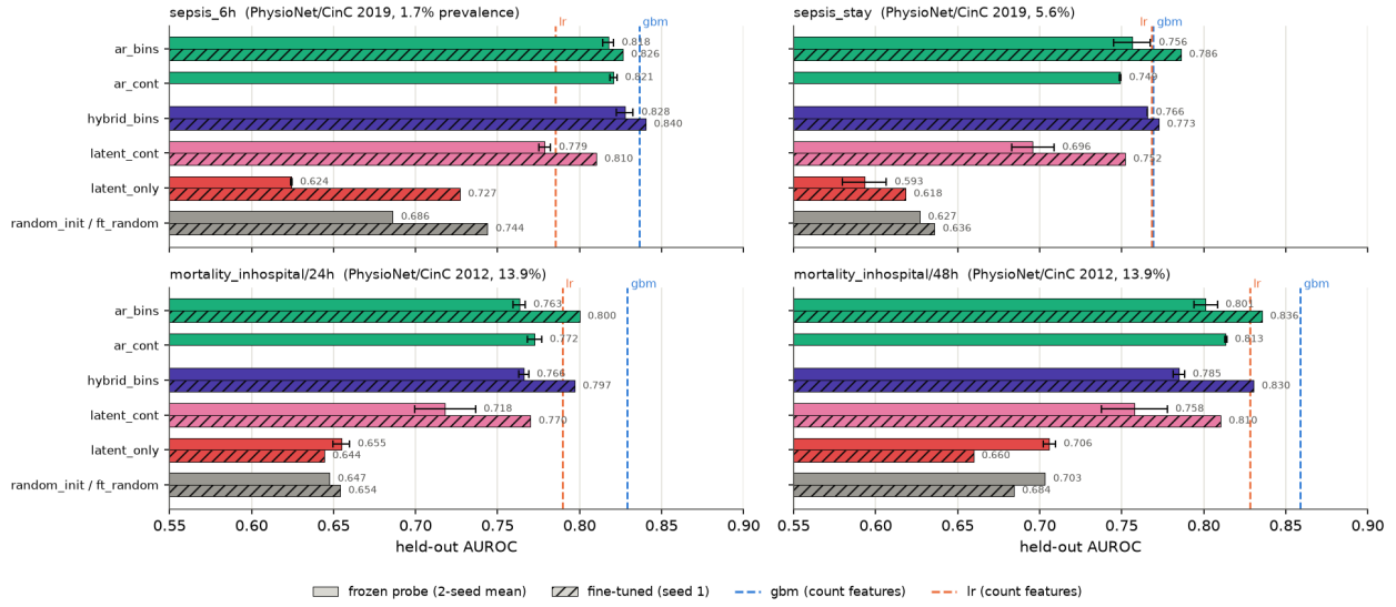
Figure 9: The four panels of the pre-registered test, one per task. Solid bars are the frozen-probe two-seed mean with a min-max whisker across the two seeds; hatched bars are the end-to-end fine-tuned point on the seed-1 checkpoint (a single seed, so no whisker). Dashed lines mark gbm and lr on that task’s own held-out split. Rendered by scripts/plot_a2.py from the committed summary.md tables.
