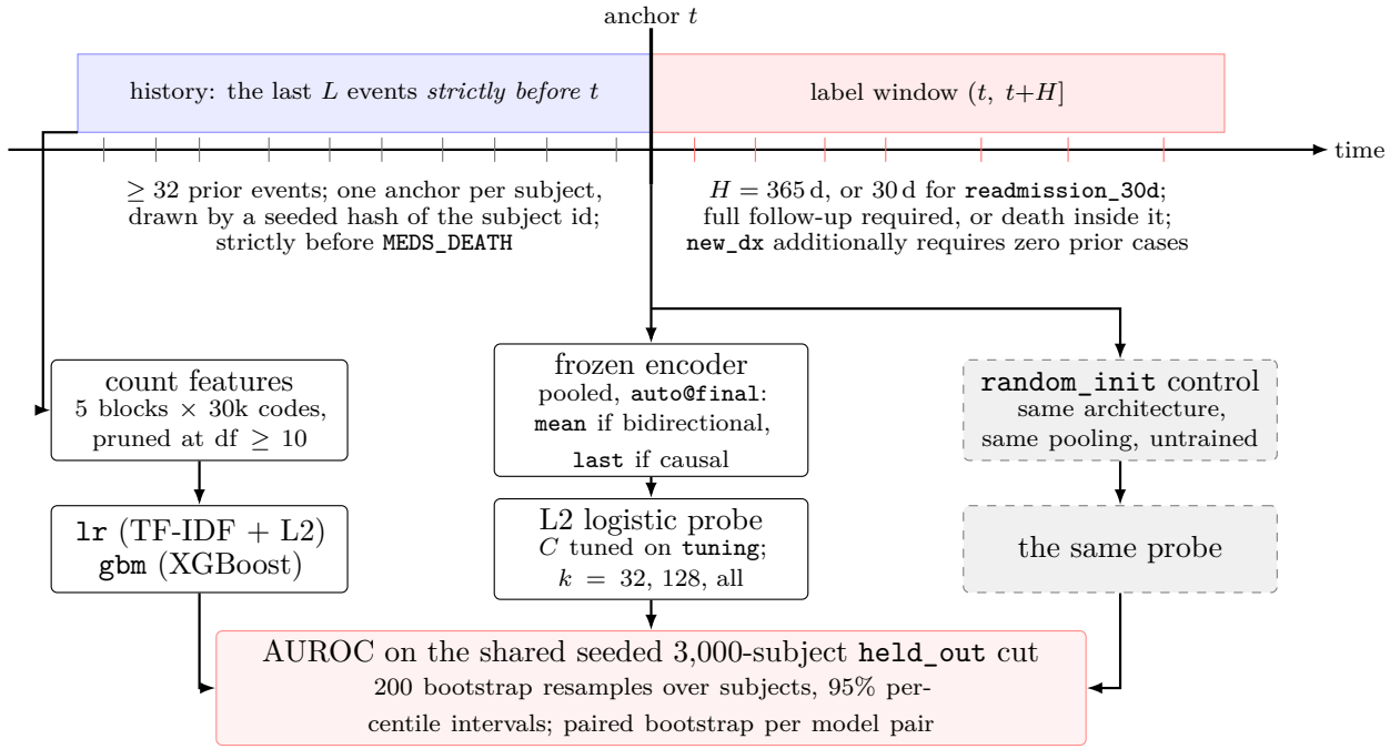
Figure 3: The evaluation protocol. Every model in a run — count baselines, frozen-encoder probes, and the untrained control — is fit and scored on identical anchors and identical rows, which is what makes the paired bootstrap legitimate and stops a checkpoint from looking better on an easier subset.
