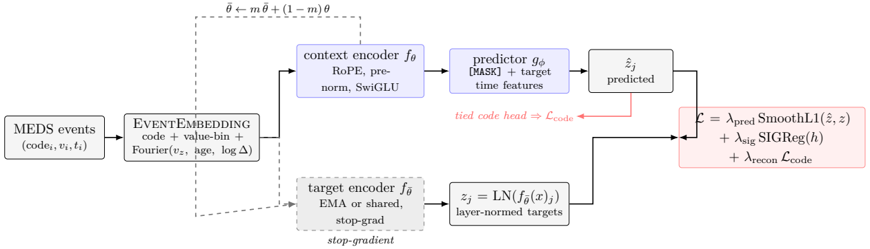
Figure 1: The shared architecture. The context encoder f_\theta and the predictor g_\phi carry gradients; the target encoder f_{\hat{\theta}} runs under stop-gradient, either as a weight-shared copy or as an EMA copy, and is never told what code or value the masked span holds. Nothing is reconstructed in input space by the latent term; the optional code-reconstruction term \mathcal{L}_{\text{code}} passes the predicted latent through the tied code head.
