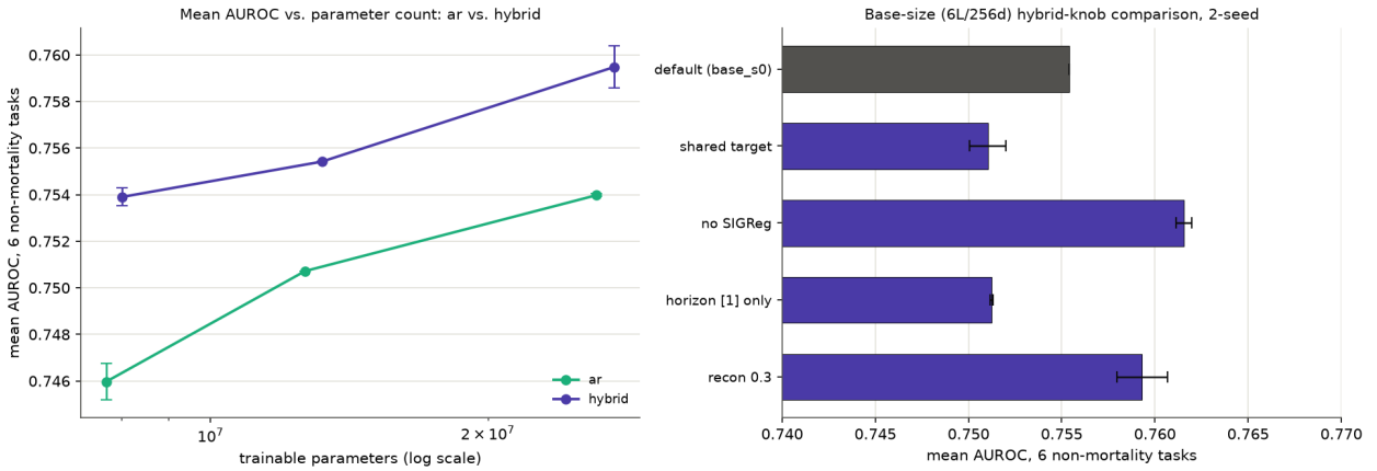
Figure 8: Left: mean AUROC across the six non-mortality tasks against trainable parameter count (log x ) for ar and the hybrid across the three sizes, with 2-seed min-max error bars (none at base, seed 0 only). Right: the base-size hybrid-knob comparison as horizontal bars with 2-seed min-max whiskers (none for the default row). Regenerated by scripts/plot_ablate2.py , which builds each model from its config overrides to compute the parameter counts rather than reading a hand-typed estimate.
