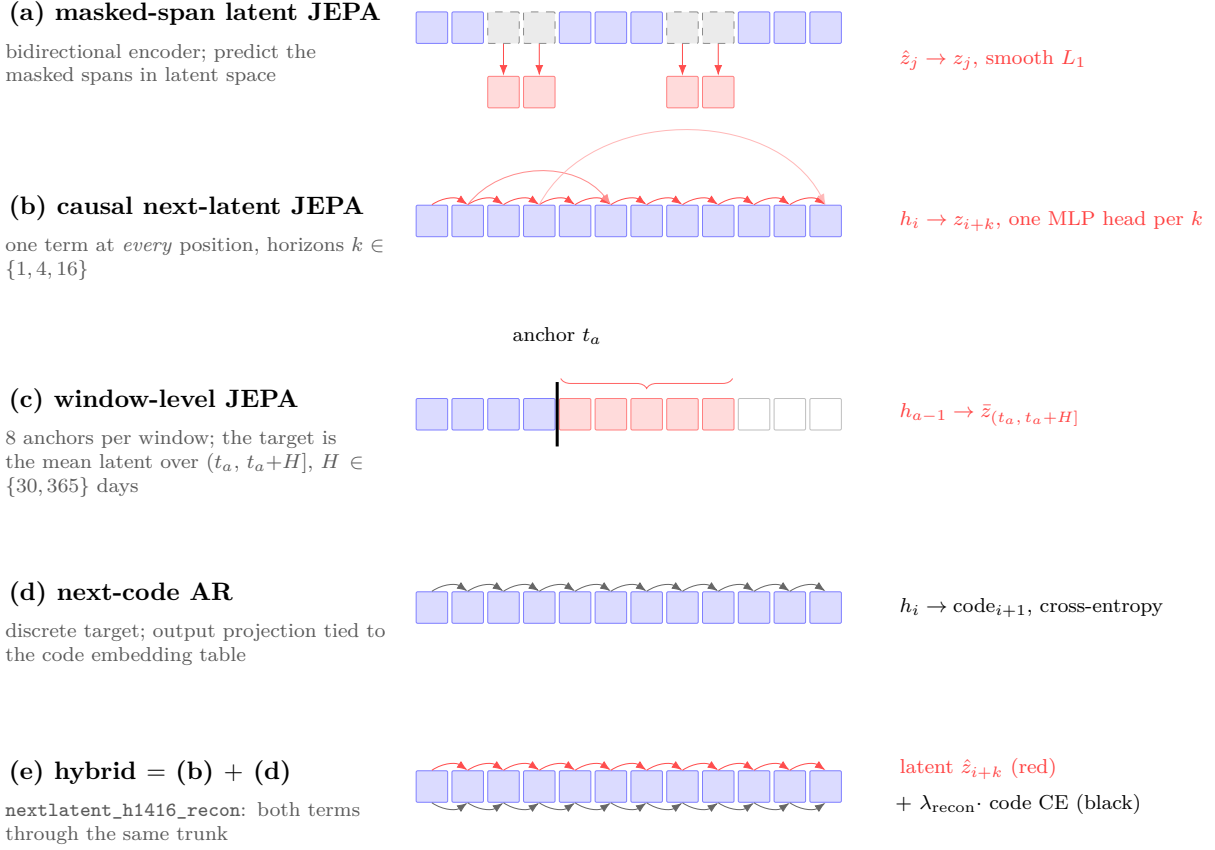
Figure 2: The five objective families, drawn on a common 12-token strip. Blue is observed context, red is a predicted or supervised position, grey dashed is masked. The difference between (a) and (b)–(e) that the experiments turn on is density : (a) places a loss term only at the 10–30% of positions a mask covers, while (b), (d) and (e) place one at every position.
