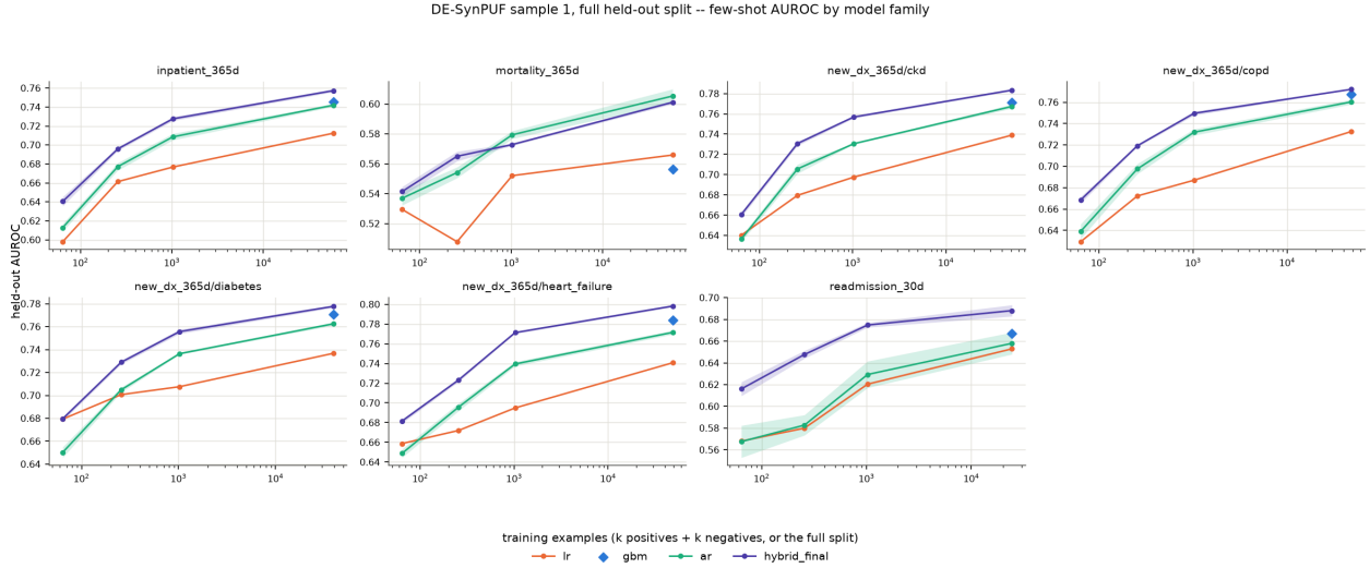
Figure 6: Held-out AUROC against few-shot training size, full held-out split, one panel per task, one line per model family.
