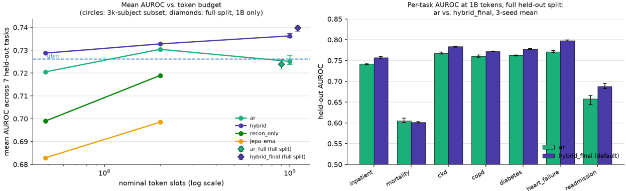
Figure 7: Left: mean AUROC against token budget (log x ) for ar , the hybrid, recon_only and jepa_ema on the 3,000-subject held-out subset (circles), with gbm as a horizontal reference; the subset 1B ar /hybrid points are 3-seed means with a min-max error bar. The diamonds at 1B are the full-held-out-split (Section 6.10) 3-seed means for ar and hybrid_final , offset in x so they do not overlap the subset circles. Right: per-task AUROC at 1B tokens on the full held-out split, ar against hybrid_final , paired bars, each a 3-seed mean with a min-max whisker.
