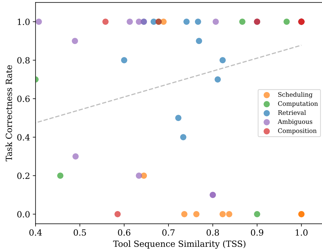
TSS vs Correctness ( r=0.32 , p=0.005 )
