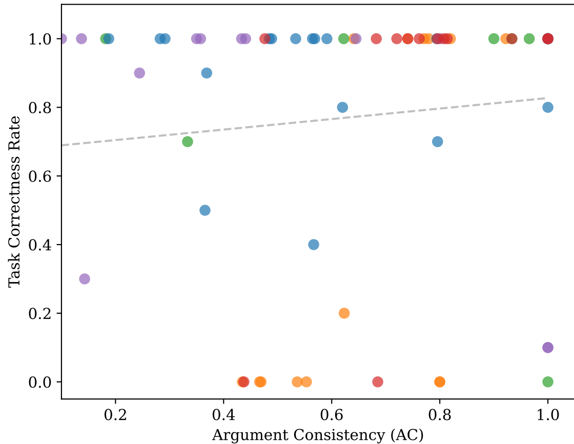
AC vs Correctness ( r=0.12 , p=0.311 )
