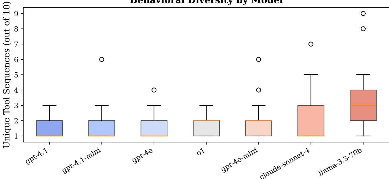
Behavioral Diversity by Model
