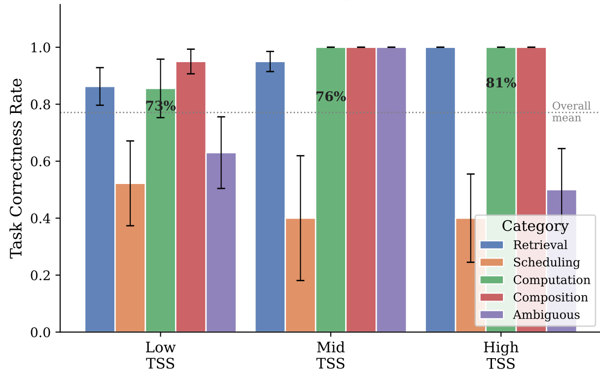
TSS vs. correctness ( r = 0.06 , p = 0.560 ; Spearman \rho = 0.22 )
