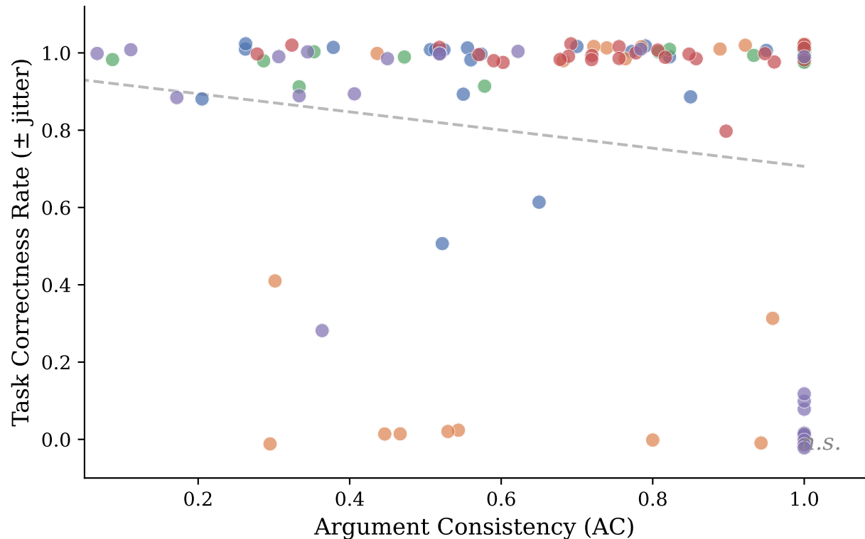
AC Does Not Predict Correctness ( r = -0.17 , p = 0.070 , n.s.)
