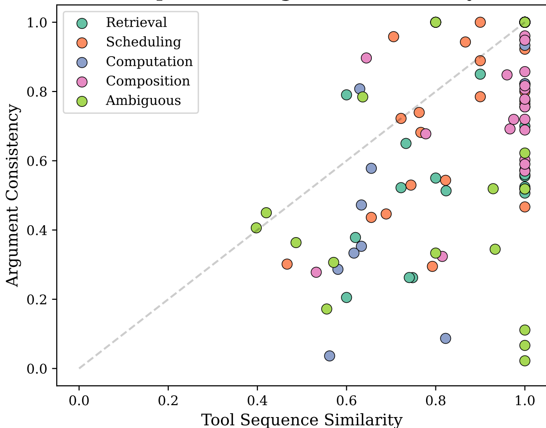
Sequence vs. Argument Consistency
