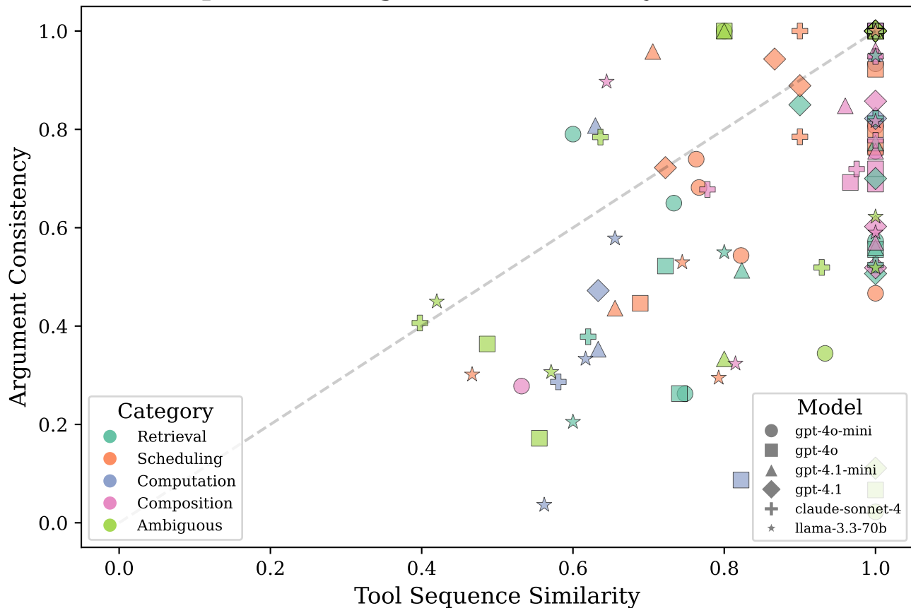
Sequence vs. Argument Consistency (All Models)
