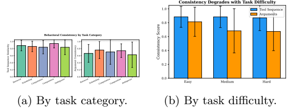
Figure 3: Ambiguous tasks show the largest (directional) consistency drop; on the fresh collection, task difficulty shows no significant effect on either metric (TSS: r = -0.04 , p = 0.67 ; AC: r = -0.15 , p = 0.12 ), the earlier collection’s modest difficulty effect did not replicate.
