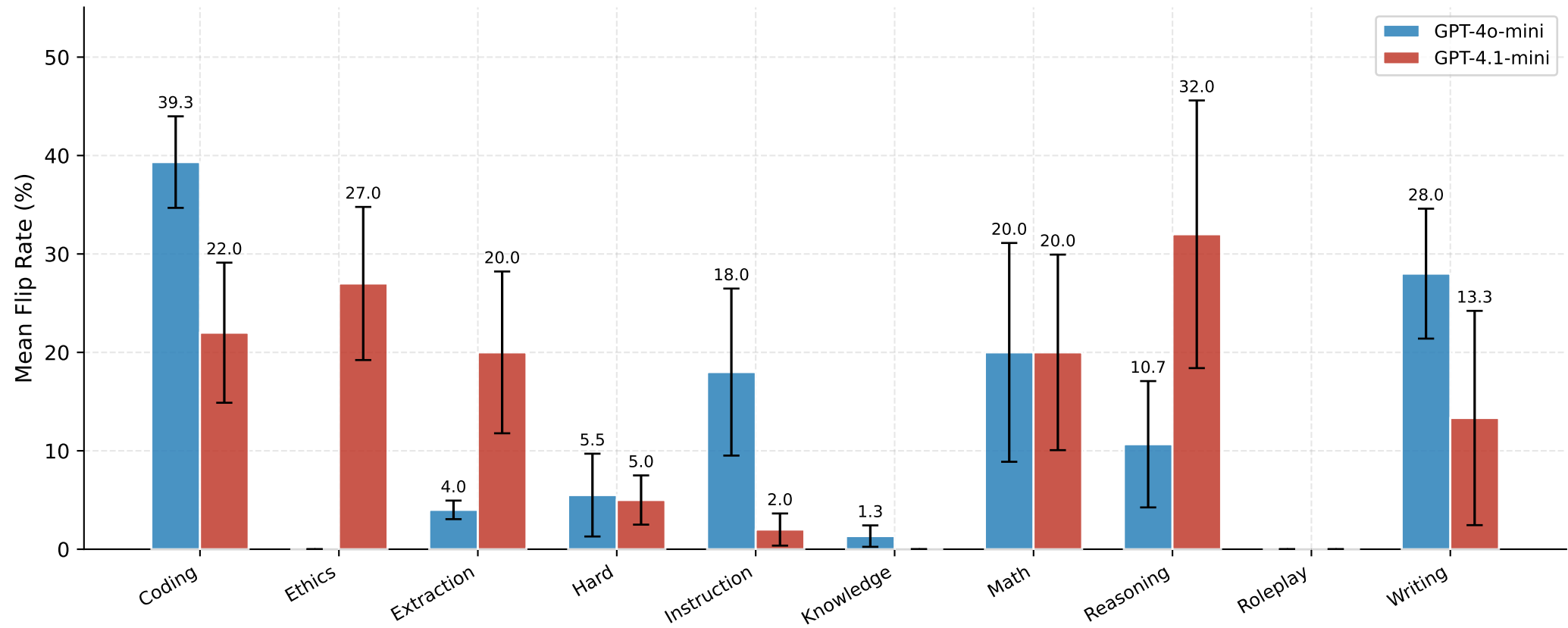
Intra-Judge Inconsistency by Task Category (error bars = \pm 1 SE)
