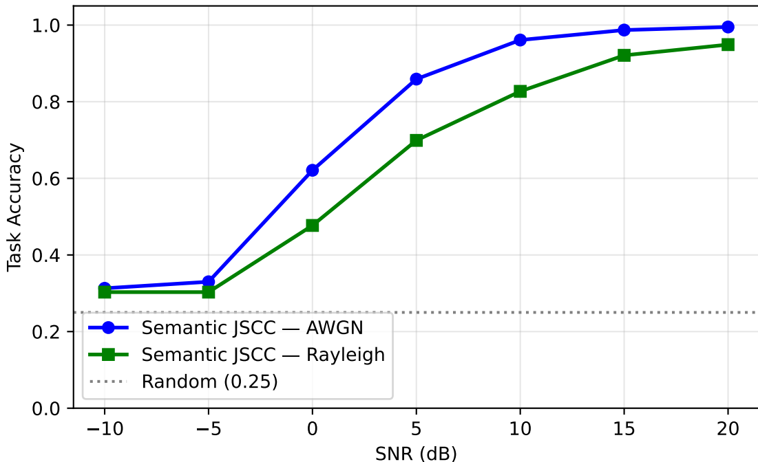
Semantic JSCC — AWGN vs Rayleigh Fading
