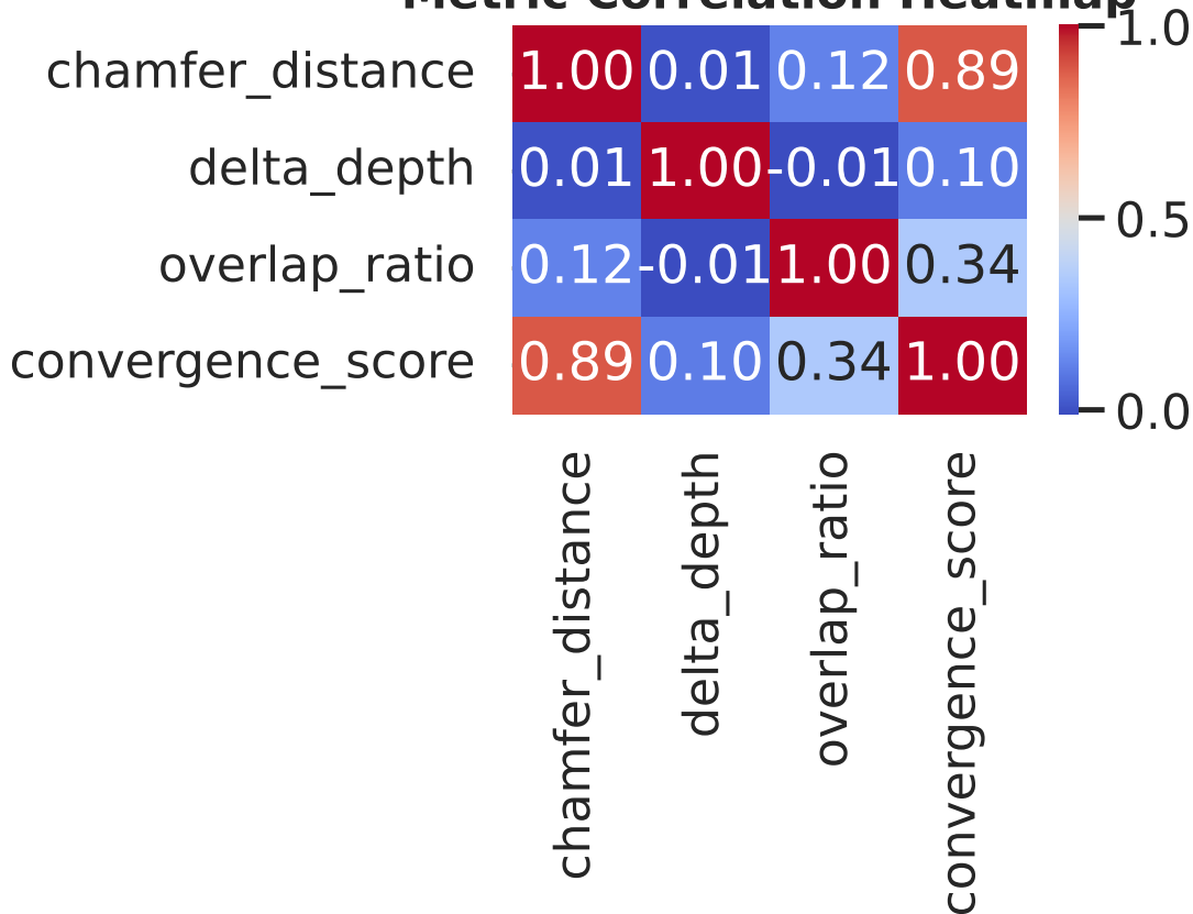
Metric Correlation Heatmap
