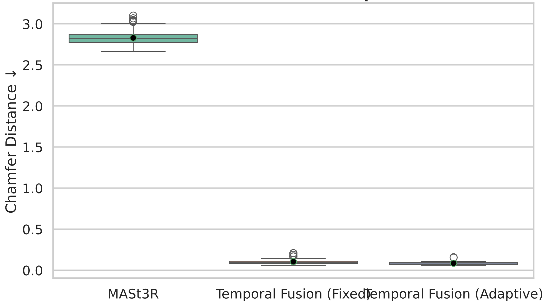
Chamfer Distance ↓ Comparison
