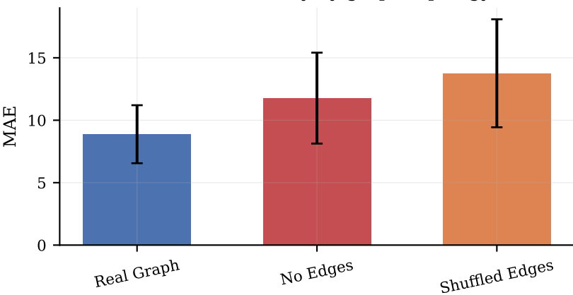
ST-GNN accuracy by graph topology
