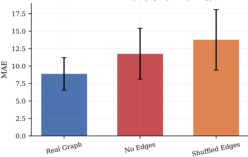
ST-GNN accuracy by graph topology
