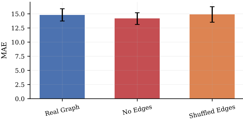
ST-GNN accuracy by graph topology
