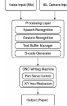
Fig. 2: CNC machine flow diagram.
