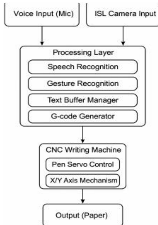
Fig 3 CNC writing flow and motion execution sequence
