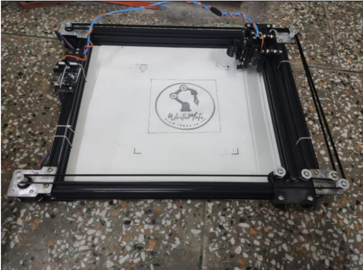
Fig 1 WriteMate prototype and major hardware units
