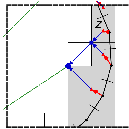
(b) The upwards translation process, where the multipole expansion of the boundary element is translated up to the leaf node's center, and then up to the parent node's center with the M2M translation, before being translated to the far-field node's center with the M2L translation.
