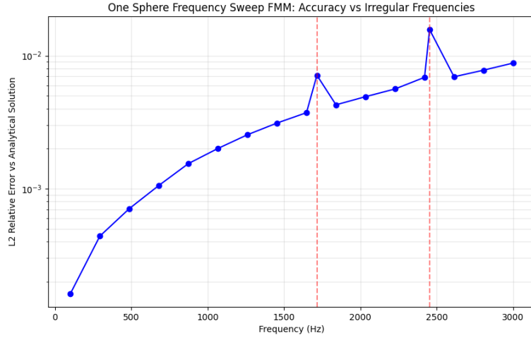
Figure 5.3.: L2 error plot for the FMM without BM formulation. We can see the error spiking as we approach the characteristic frequencies.
