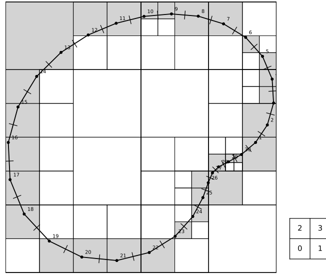
Figure 3.2.: An example of a 2D domain with a 1D boundary being split up into a Quadtree. The small square on the side shows the numbering scheme for the child cells of any given parent cell [LN06]
