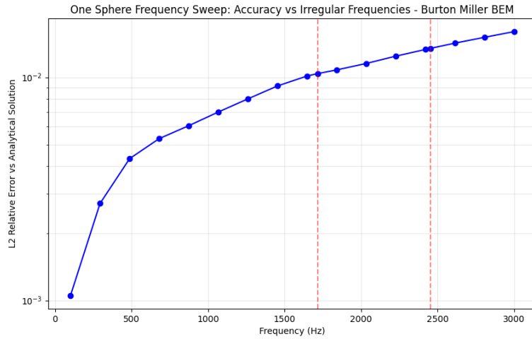
Figure 5.4.: L2 error plot for the FMM with BM formulation. We can see that there are no spikes in the error at the characteristic frequencies, demonstrating the effectiveness of the BM formulation. However, we can also see that the overall error is slightly higher than without the BM formulation, which is expected due to the reasons explained in 5.2.
