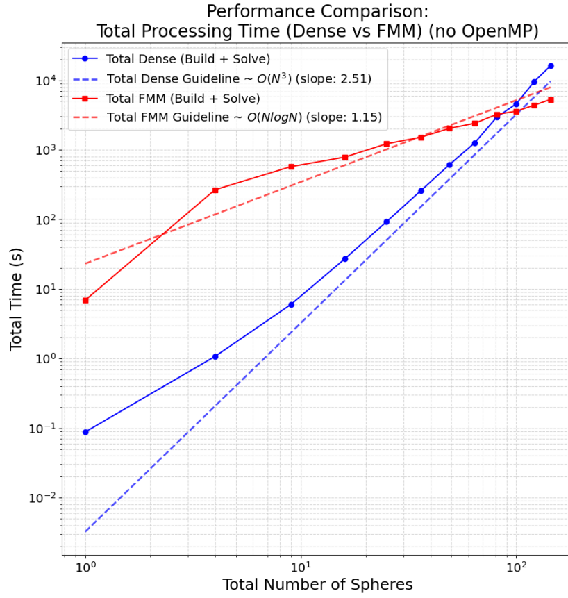
Figure 5.14.: Total time taken by the traditional BEM, as compared to the time taken by the FMM. The FMM time complexity remains the same \mathcal{O}(N \log N) in the single-threaded case, just with higher absolute times. The BEM complexity remains \mathcal{O}(N^3) .
