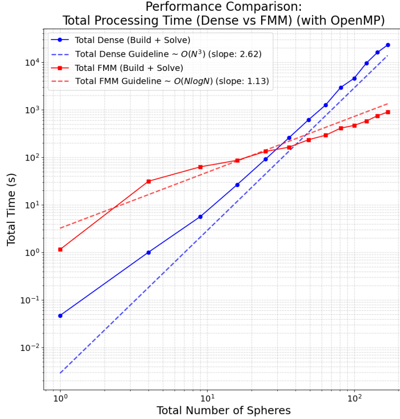
Figure 5.9.: Total time taken by the traditional BEM, as compared to the time taken by the FMM with OpenMP enabled. The log-log plot enables us to compare the scaling of the two methods. We can see that the FMM scales as \mathcal{O}(N \log N) , while the traditional BEM scales as \mathcal{O}(N^3) . The computed slope differs a bit from the theoretical slope, but we can see for the BEM it matches the \mathcal{O}(N^3) slope in the asymptote. Meanwhile, the FMM may be closer to \mathcal{O}(N) than \mathcal{O}(N \log N)
