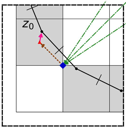
(a) We can see how the incoming information from the M2L interactions is translated down to the leaf node, and the L2P local expansion translates it onto the boundary element.
