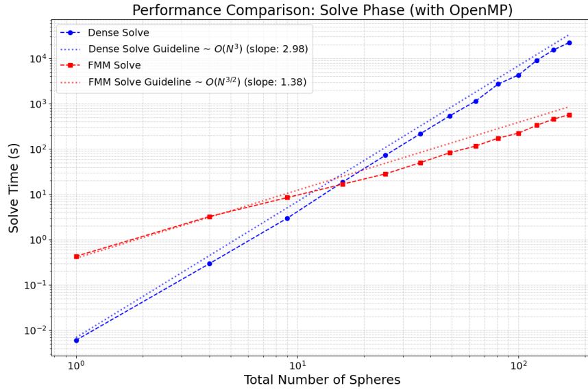
Figure 5.11.: Time taken to solve the system for the traditional BEM, as compared to the time taken to solve the FMM system. The FMM with its iterative GMRES coupled with the fast matrix-vector products scales as \mathcal{O}(N^{\frac{3}{2}}) , while the direct solver for the traditional BEM scales as \mathcal{O}(N^3) . The Direct BEM solver uses matrix inversion to solve the system, which is quite an expensive operation.
