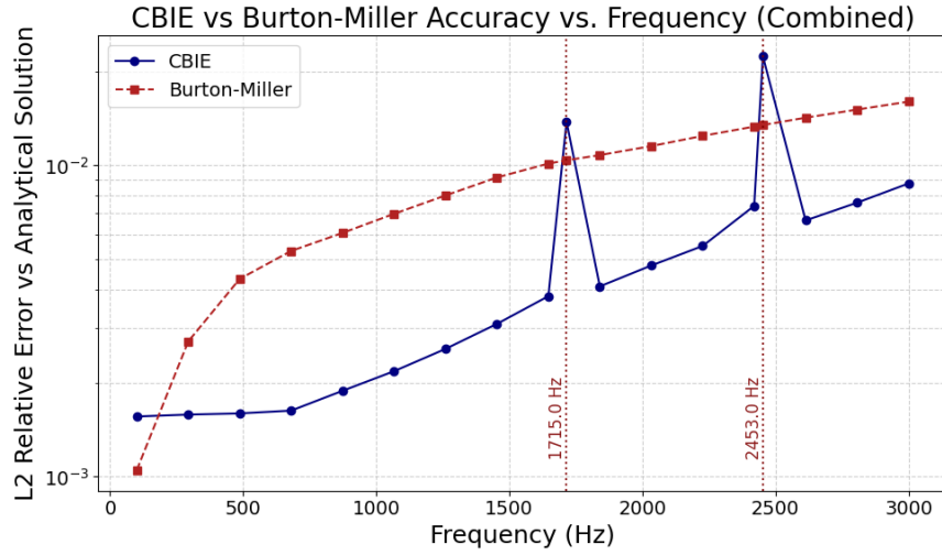
Figure 5.3.: Relative L_2 error of the numerical solution compared to the analytical solution for a frequency sweep from 100Hz to 3000Hz, both with, and without using the BM formulation. The spikes in the error of the CBIE at the characteristic frequencies (1715 Hz and 2453 Hz) demonstrate the non-uniqueness issue at these frequencies. While the BM displays no such spikes, its overall error is higher than the CBIE formulation, due to the stronger singularity of the HBIE kernel compared to the CBIE kernel.
