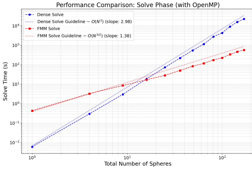
Figure 5.10.: Time taken to solve the system for the traditional BEM, as compared to the time taken to solve the FMM system. The FMM with its iterative GMRES coupled with the fast matrix-vector products scales as \mathcal{O}(N^{\frac{3}{2}}) , while the direct solver for the traditional BEM scales as \mathcal{O}(N^3) . The Direct BEM solver uses matrix inversion to solve the system, which is quite an expensive operation.
