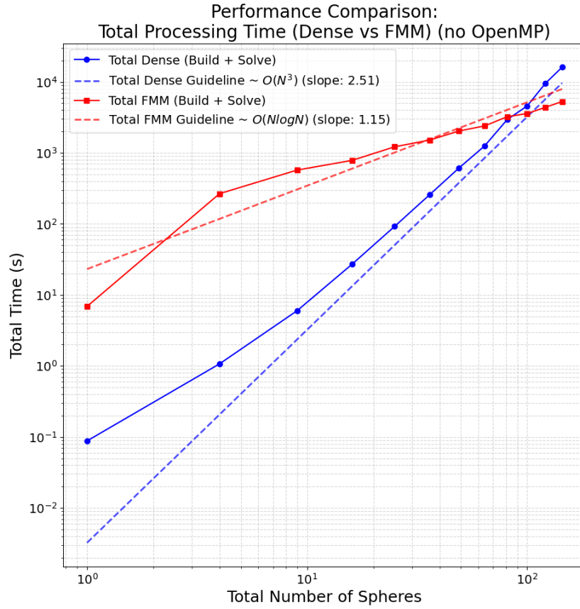
Figure 5.7.: Total time taken by the traditional BEM, as compared to the time taken by the FMM.
