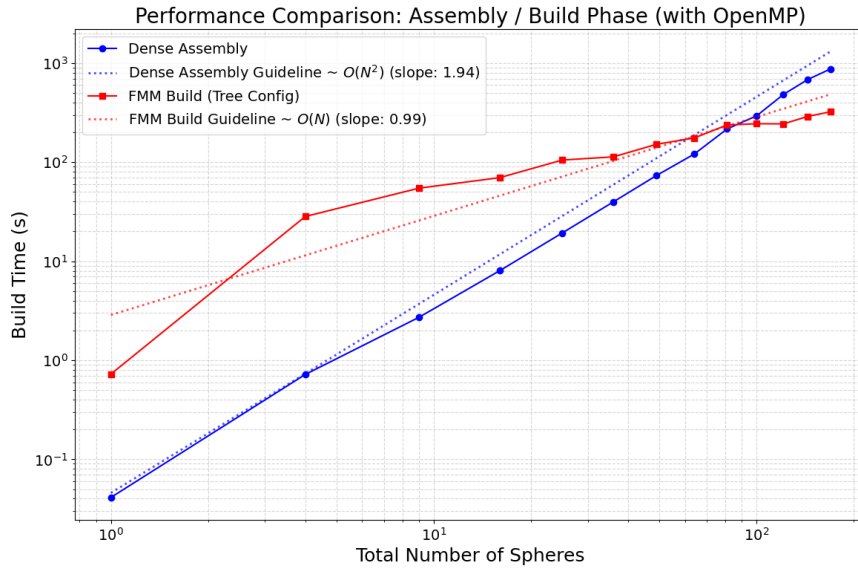
Figure 5.9.: Time taken to set up the system matrix for the traditional BEM, as compared to the time taken to set up the FMM data structures and precompute the translation operators. The Dense BEM matrix assembly takes \mathcal{O}(N^2) time, while the FMM build time scales as \mathcal{O}(N) .
