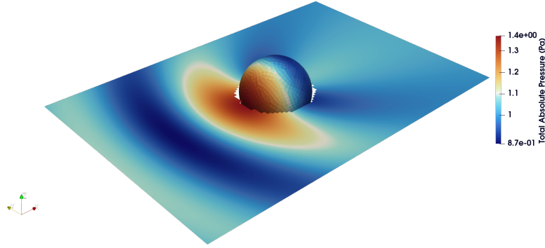
Figure 5.1.: Numerical solution for the total absolute pressure field on a slice on the z = 0 plane and on the scatterer itself. The spherical scatterer is excited by a plane wave traveling in the positive x -direction, with a frequency of f = 500 Hz.
