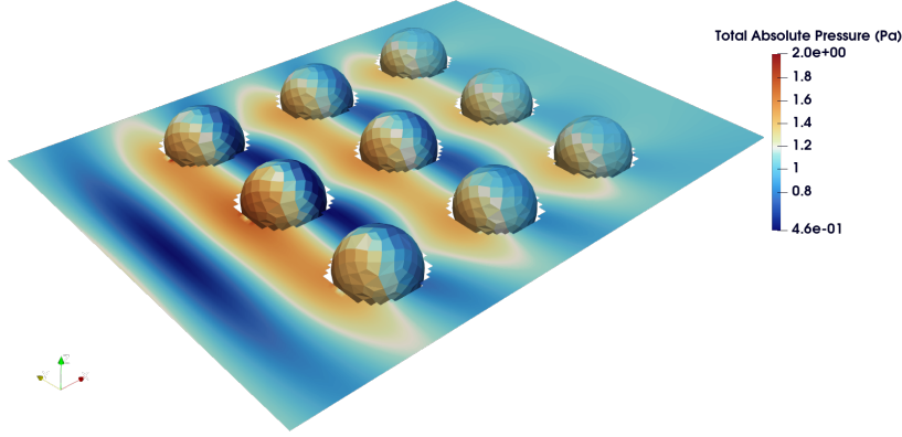
Figure 5.4.: A 3 \times 3 grid of spherical scatterers, in an incident plane wave of frequency f = 500\text{Hz} . The plot shows the Total Absolute Pressure (Pa) field on the surface of the scatterers, as well as a slice of the field on the z = 0 plane.
