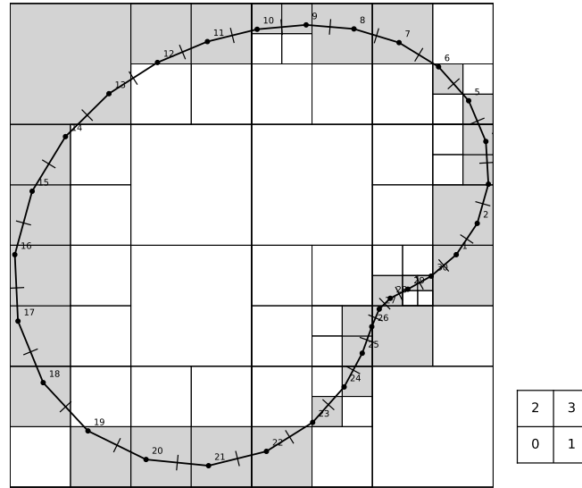
Figure 3.2.: An example of a 2D domain with a 1D boundary being split up into a Quadtree. The small square on the side shows the numbering scheme for the child cells of any given parent cell [liufastmultipoleboundary2006]
