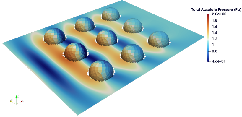
Figure 5.4.: A 3 \times 3 grid of spherical scatterers, in an incident plane wave of frequency f = 500\text{Hz} . The plot shows the Total Absolute Pressure (Pa) field on the surface of the scatterers, as well as a slice of the field on the z = 0 plane.
