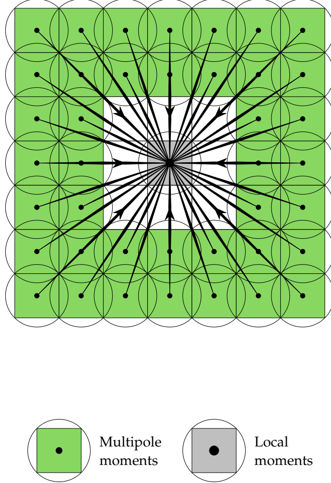
Figure 4.2.: A 2D representation of the M2L interaction list. In 3D, there are 7^3 - 1 = 342 possible relative positions for the M2L interactions. [kohnkecudafastmultipole2021]
