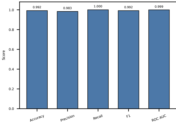
Gradient Boosting Fall-Detection Performance
