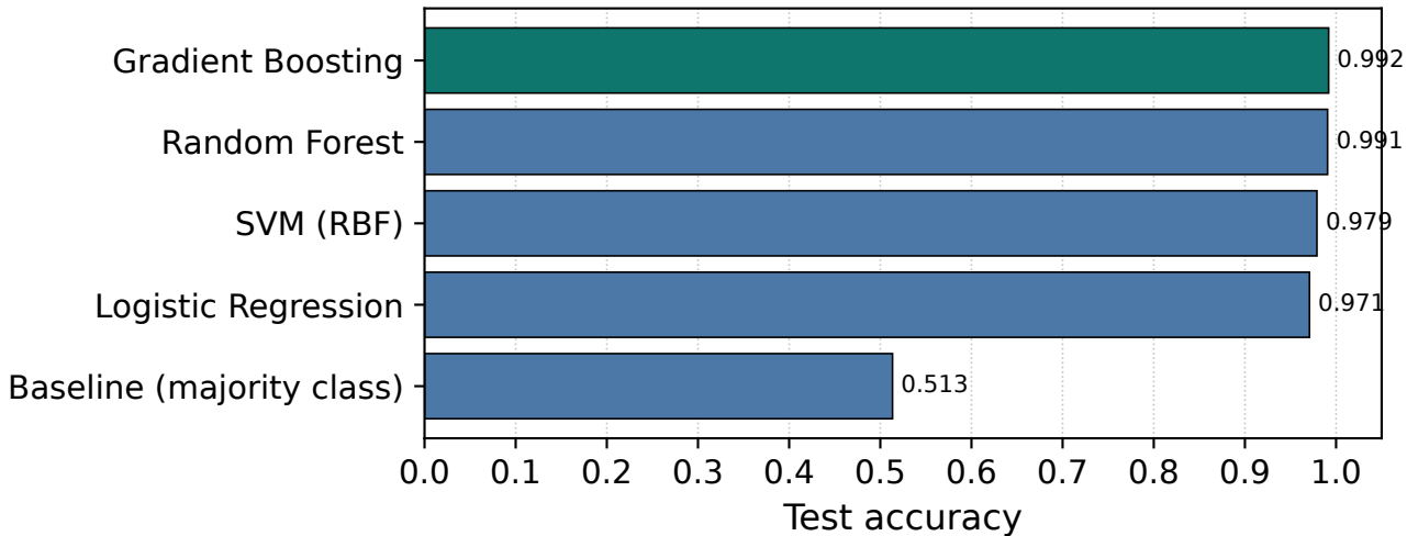
Fall-Detection Model Test Accuracy
