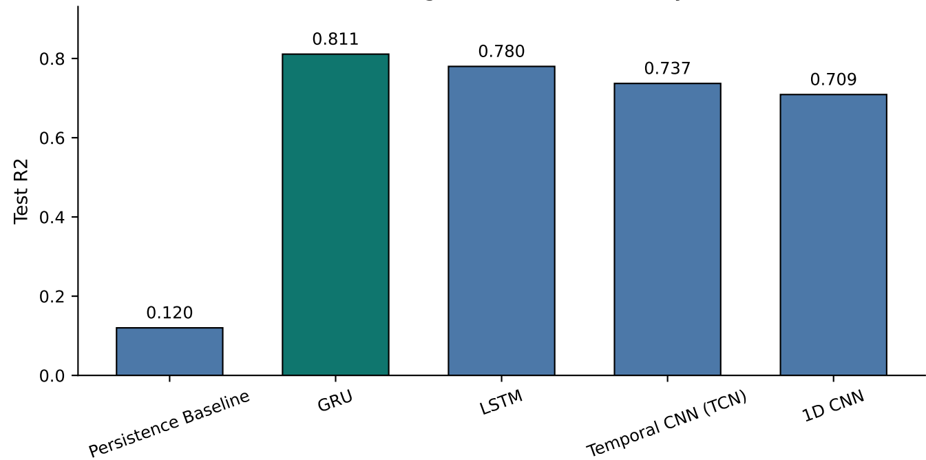
CO Forecasting Model Test Accuracy (R2)
