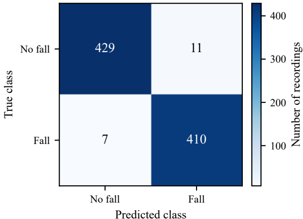
SVM Test-Set Confusion Matrix
