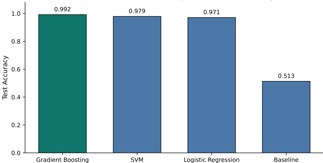
Fall-Detection Model Comparison: Test Accuracy
