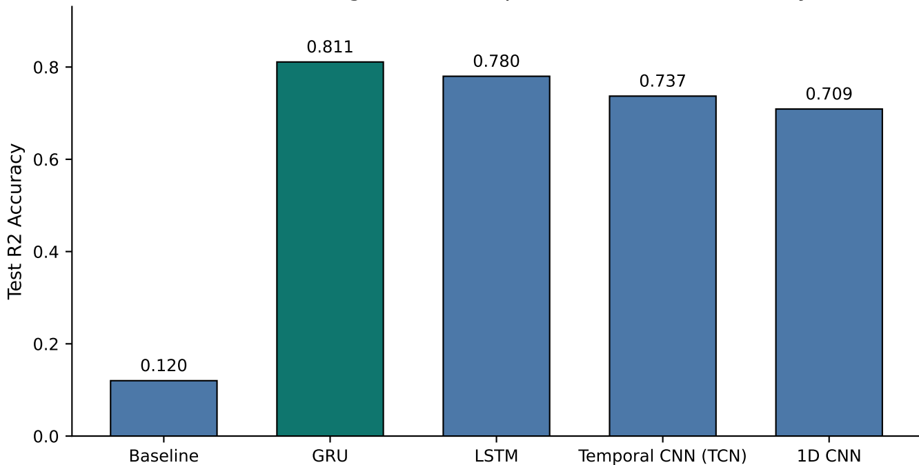
CO Forecasting Model Comparison: Test R2 Accuracy
