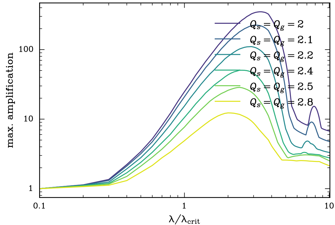
Maximum swing amplification at r = 1.0 (thin disk)
