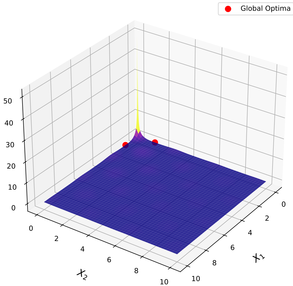
3D Surface with Global Optima
