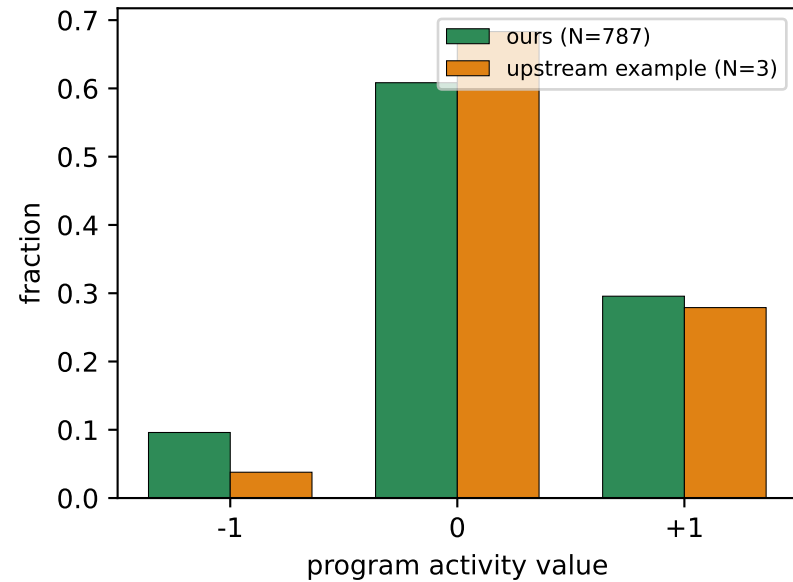
A. Activity distribution (mean ours=0.20)
