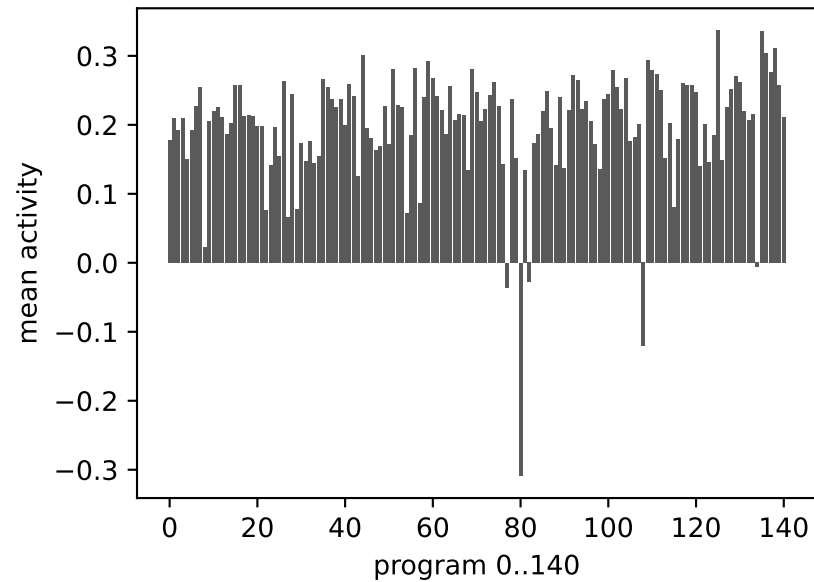
B. Per-program mean activity
