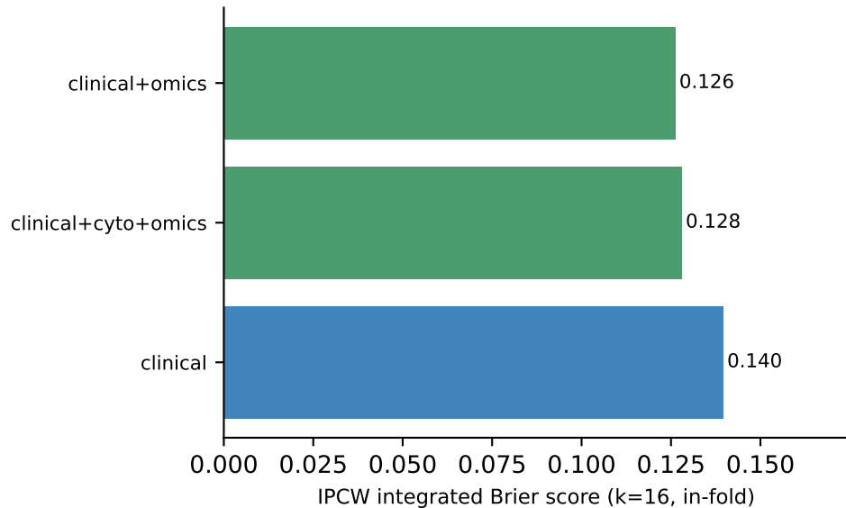
B. IPCW-IBS by model class (lower=better)
