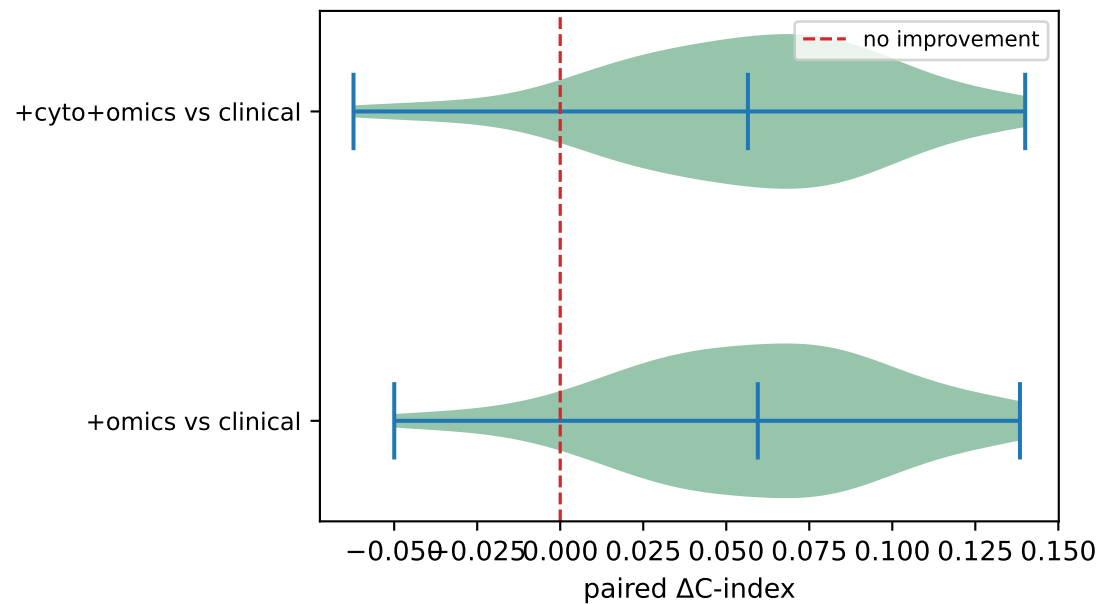
B. Paired \Delta C distribution
