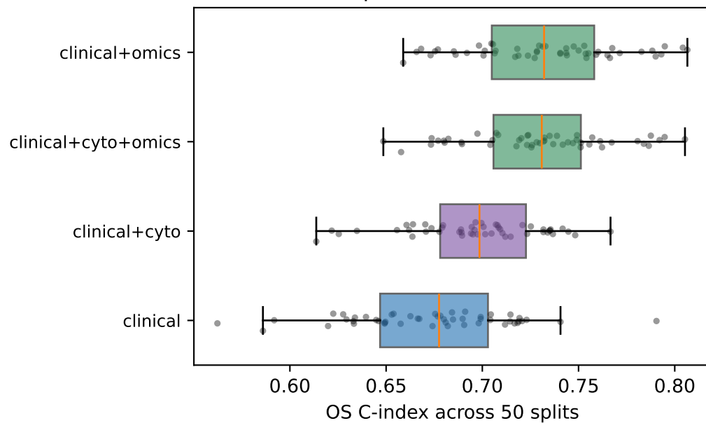
A. Per-split C-index distribution
