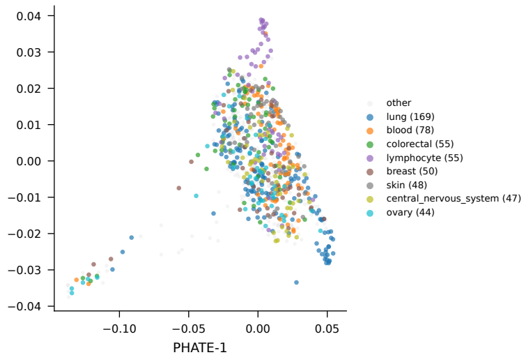
Lineage (PHATE)
