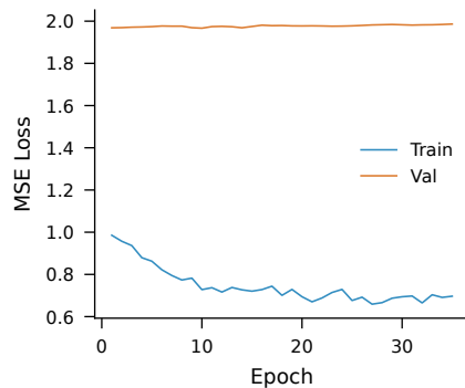
PRECISE (35 epochs)
