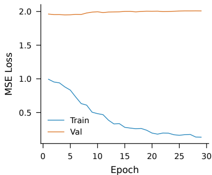
TCRP (29 epochs)
