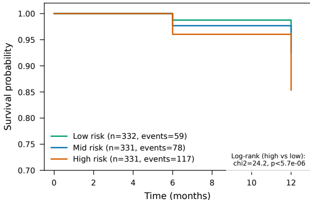
KM Curves by LOO Risk Tertile (TT2L)
