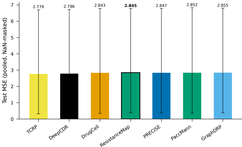
Drug Response Prediction: SOTA Benchmark
