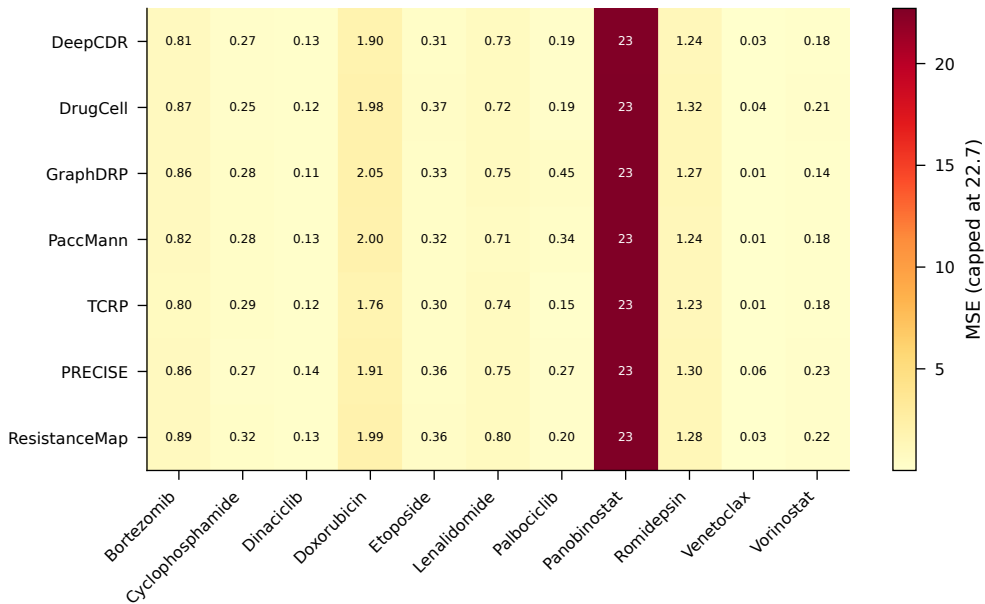
Per-Drug Test MSE by Model
