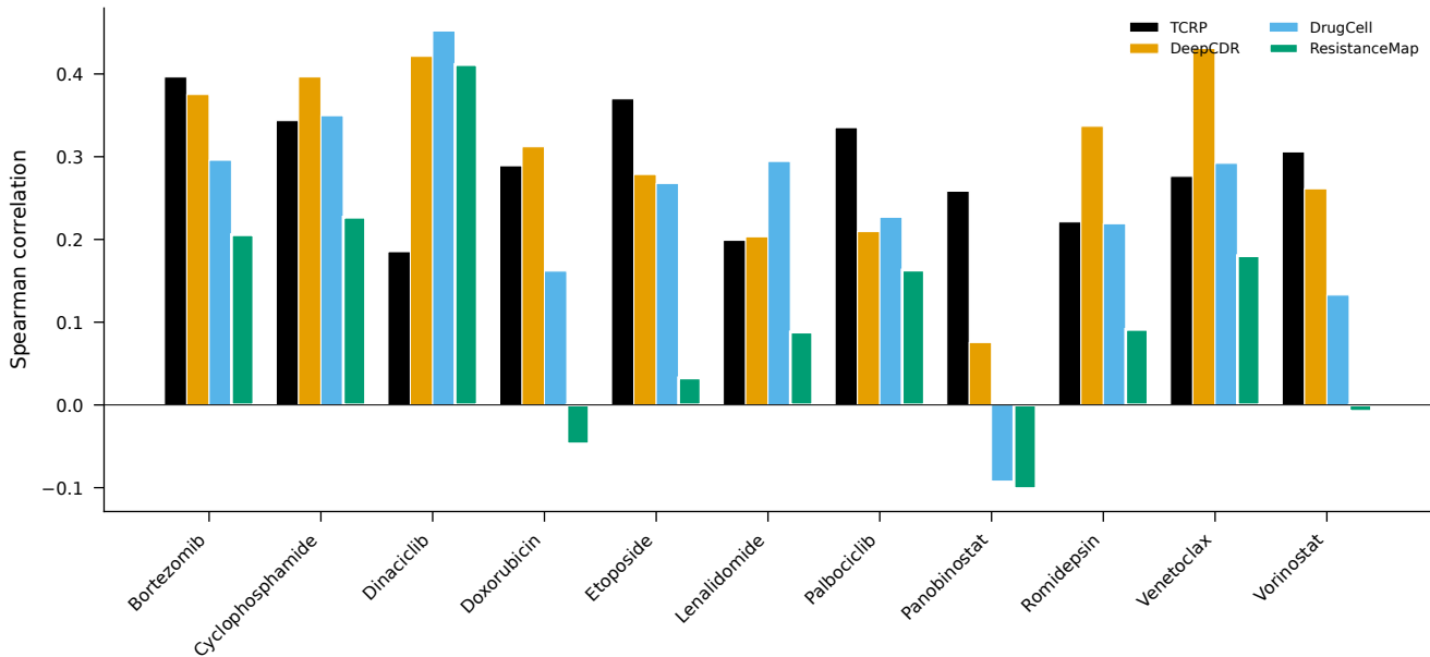
Per-Drug Spearman: ResistanceMap vs Top SOTA Models
