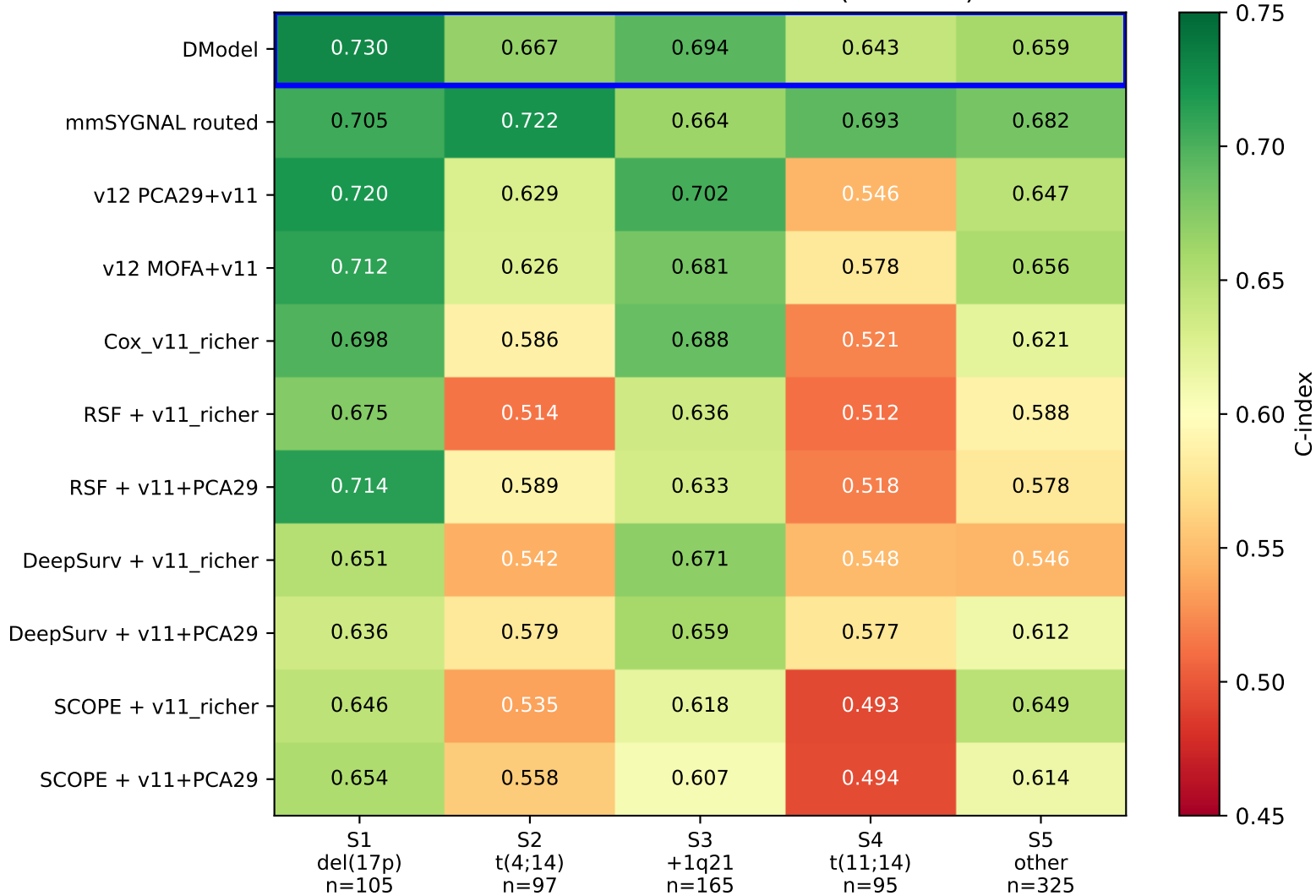
Per-stratum C-index across all models — DModel (blue box) vs literature SOTA
