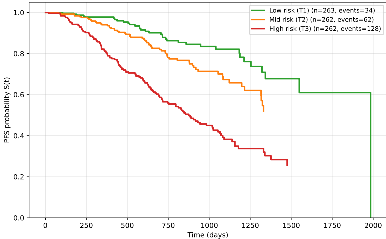
Kaplan-Meier curves by DModel predicted-risk tertiles MMRF N=787 (LOO log-hazards)
