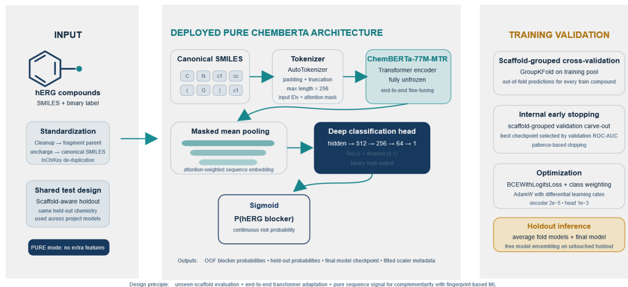
Figure 4. FT-ChemBERTa: SMILES sequence \rightarrow tokens \rightarrow fine-tuned Transformer encoder \rightarrow probability.
