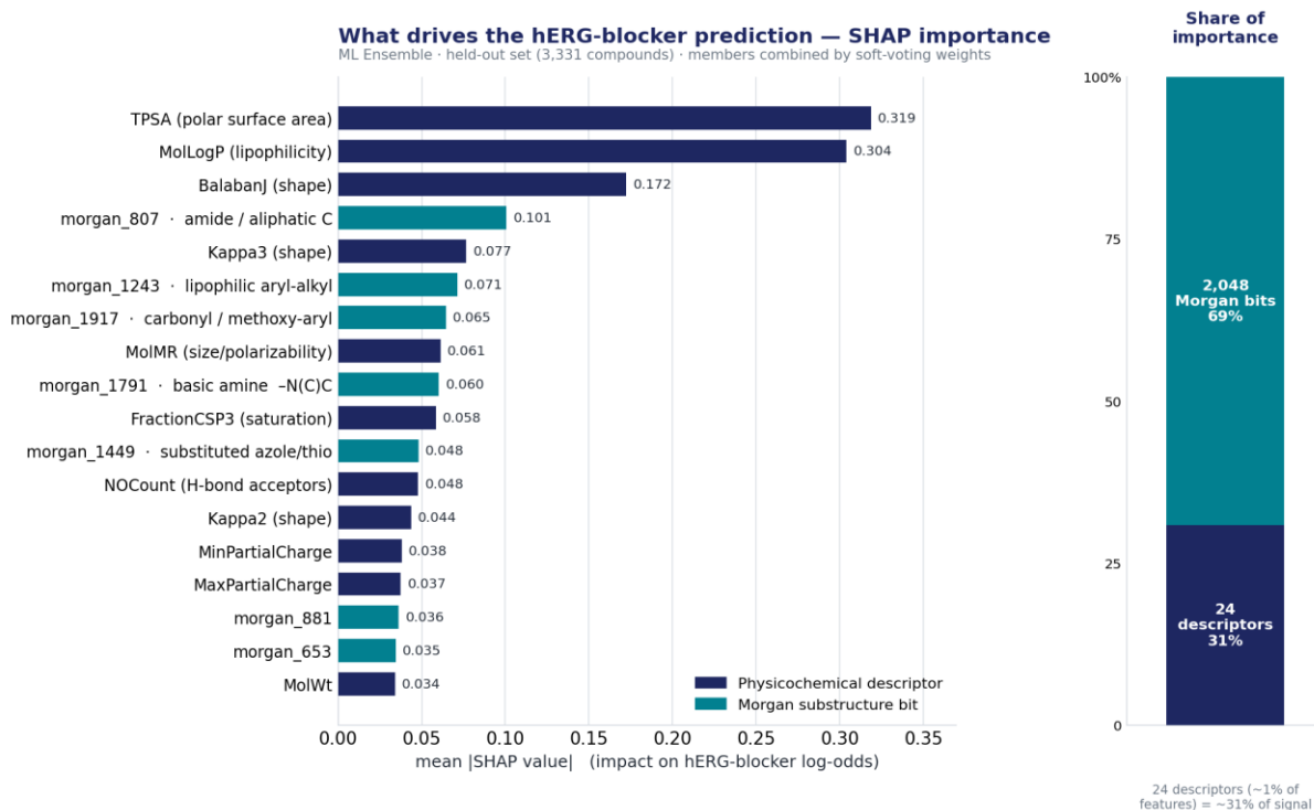
Figure 10. SHAP feature importance for the ML-Ensemble classifier on the held-out set (members combined by soft-voting weights). TPSA, MolLogP and BalabanJ dominate; the 24 descriptors (~1% of the features) carry ~31% of total importance.
