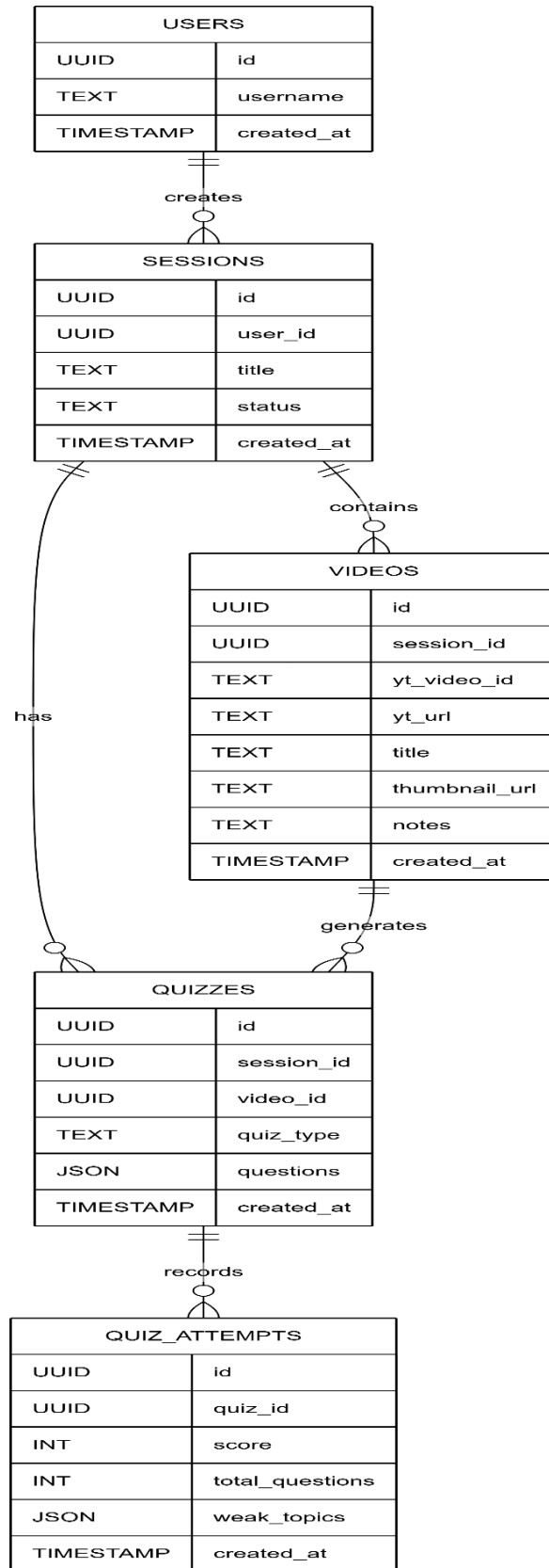
Figure 7: Database Entity-Relationship Diagram
