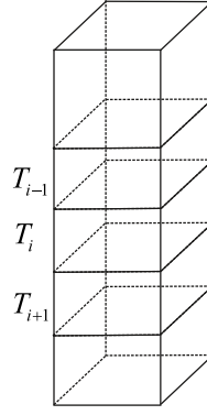
Fig. 5. Three (l, w, 1) -boxes T_{i-1}, T_i, T_{i+1} .
