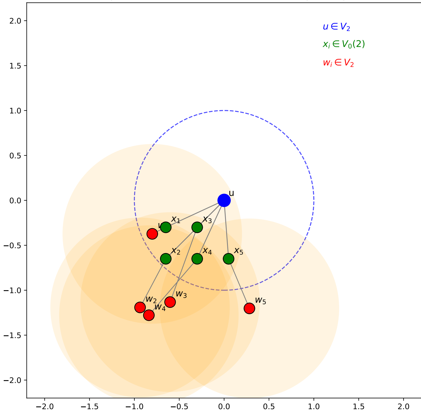
Counterexample: 5 two-demand vertices served by a single V_2 vertex
