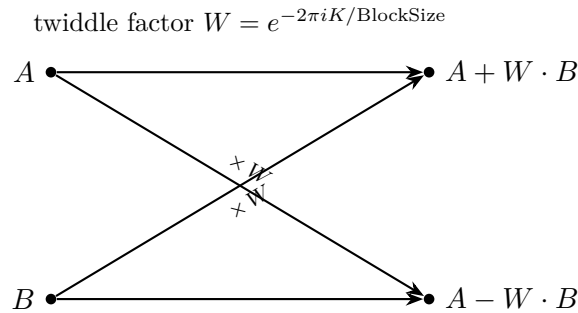
Figure 4.2: One radix-2 Cooley–Tukey butterfly. Two complex inputs A , B combine into two outputs using a single complex multiply and an add/subtract – FFTButterflyCS performs exactly this, once per grid cell, per stage, per axis.
