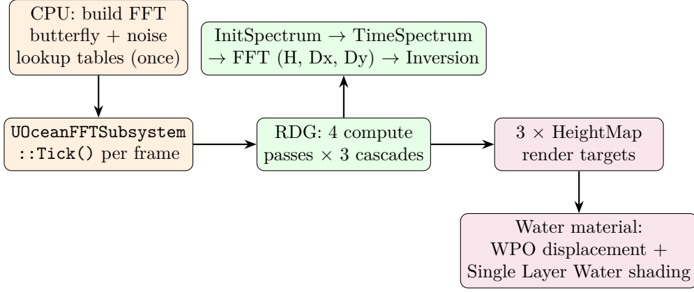
Figure 4.1: Data flow from CPU precompute through GPU simulation to the shaded pixel. The butterfly and noise lookup tables (top-left) are the only CPU-side cost; everything else happens on the GPU every frame via the Render Dependency Graph.
