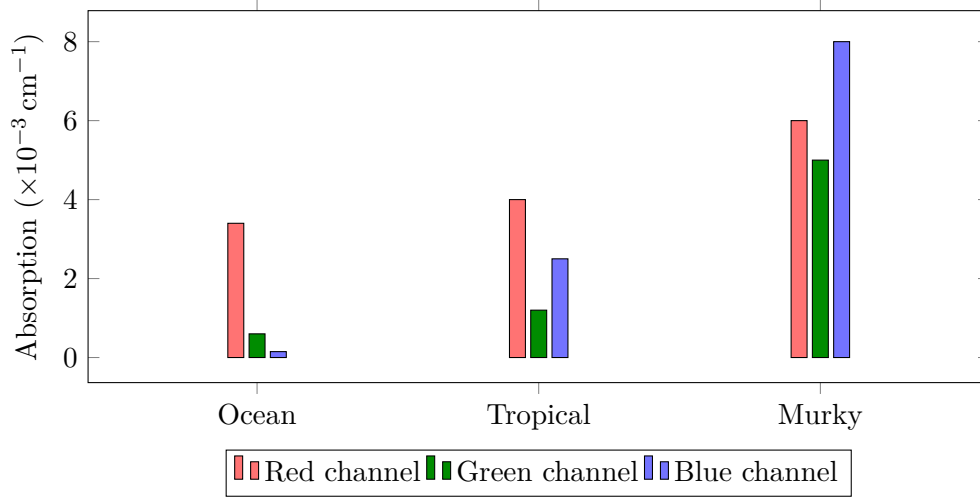
Figure 4.4: Per-channel absorption coefficients across the three presets. Ocean shows the steep red \gg green \gg blue drop-off of clear seawater; Murky is flatter and elevated across all channels, matching turbid water’s much shorter visibility depth.
