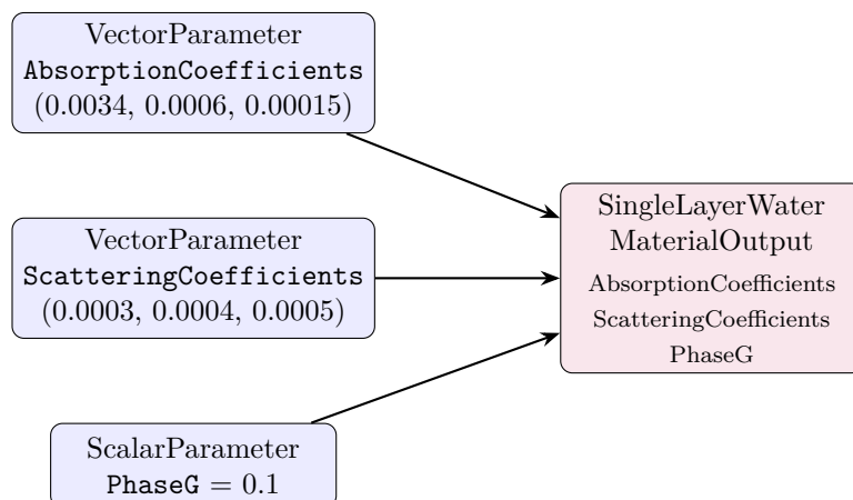
Figure 4.3: The base water-colour wiring, isolated from the rest of the material graph: three parameter nodes feeding directly into the Single Layer Water output node. Section 4.8 extends this with a blend chain in front of each pin.
