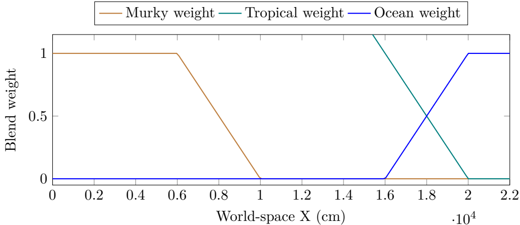
Figure 4.5: The two-stage blend ramp: Murky \rightarrow Tropical over x \in [6000, 10000] cm, then Tropical \rightarrow Ocean over x \in [16000, 20000] cm. Each preset’s optical coefficients are linearly interpolated by these weights before reaching the Single Layer Water output node.
