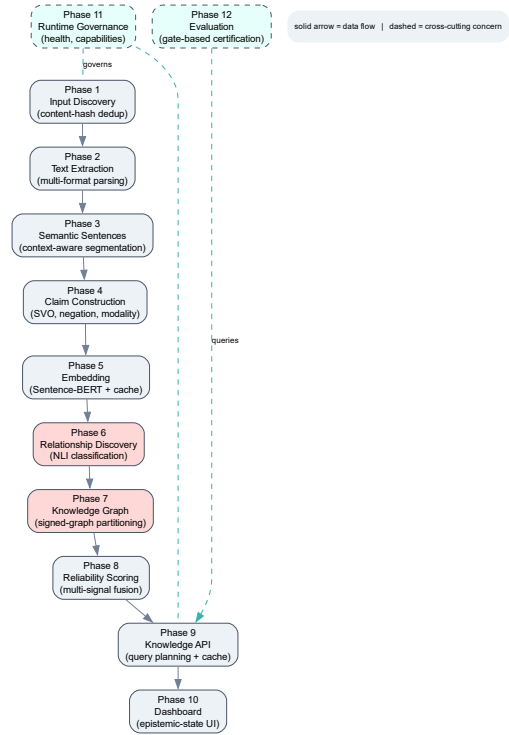
Figure 1: SMRITI’s twelve-phase pipeline. Phases 11 (runtime governance) and 12 (evaluation) are cross-cutting.
