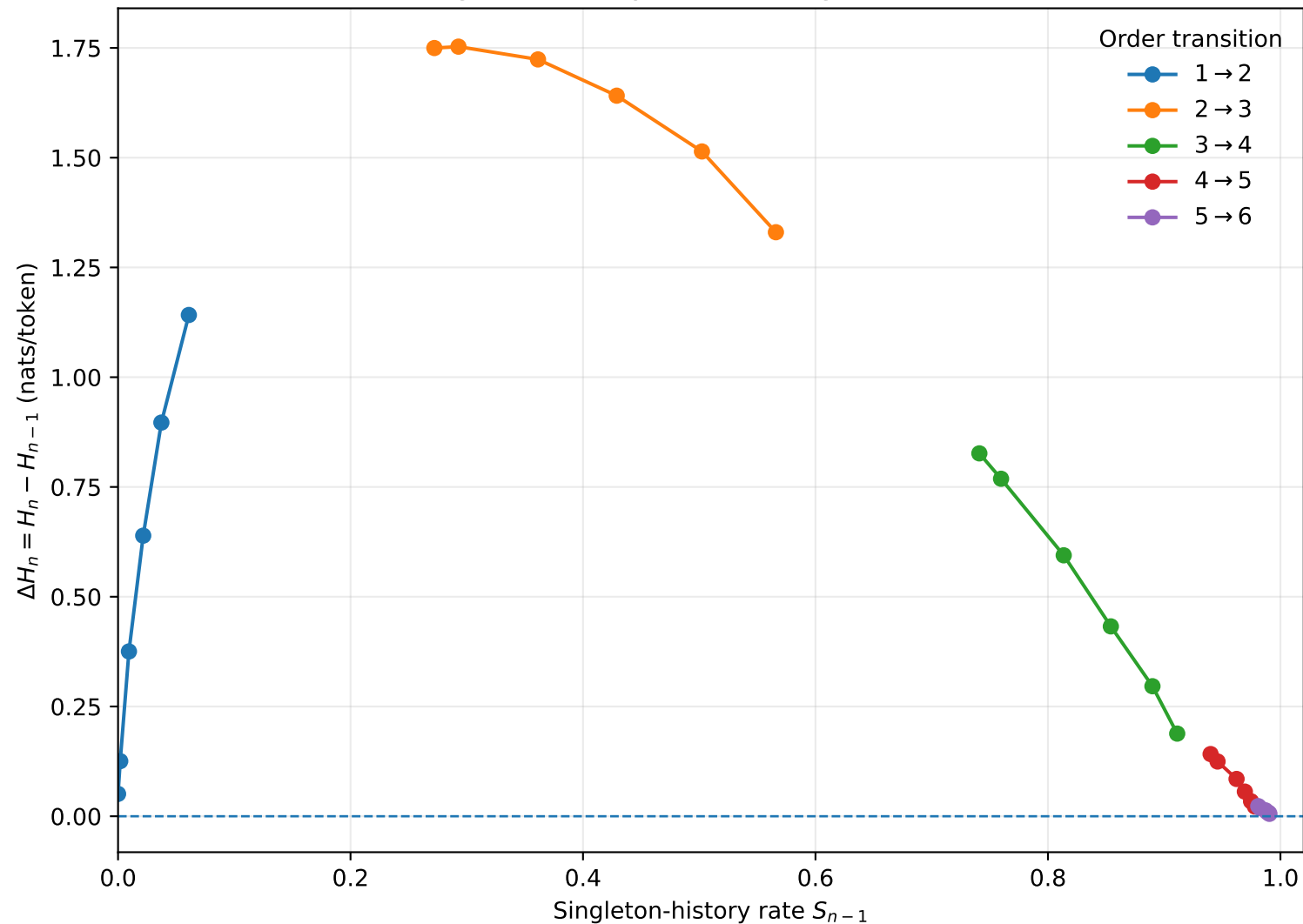
Singleton-history rate vs marginal test loss
